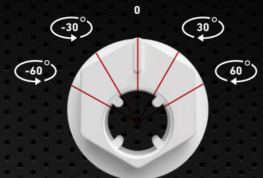
Nozzle Angle Installation Key
